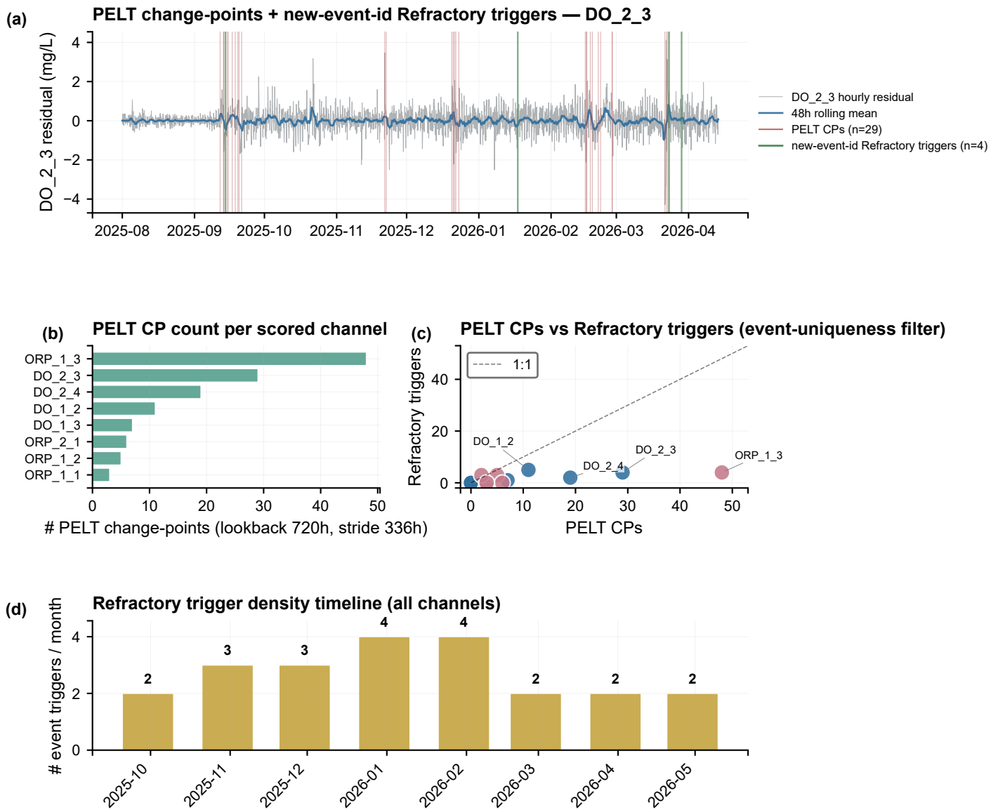
Figure V15. PELT batch calibration + event-uniqueness filter
